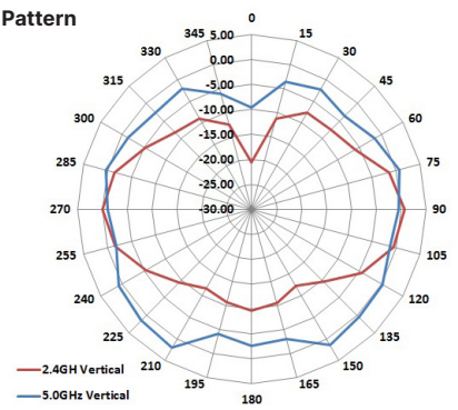
E-Plane Pattern
