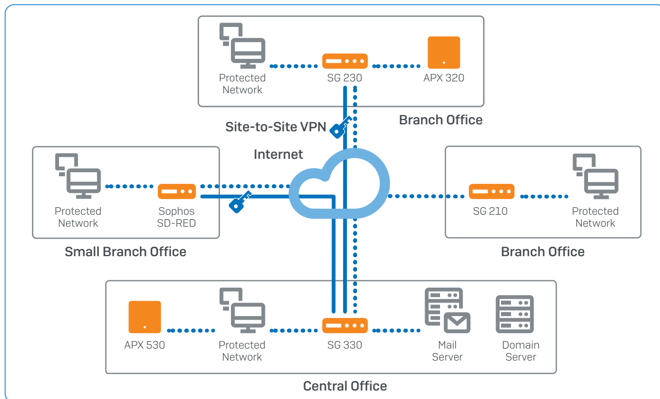
Scenario using SG Series appliances and SD-WAN for branch offices
