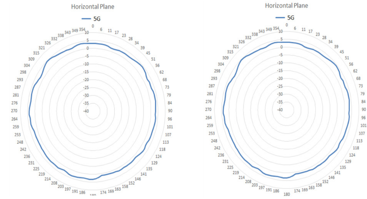
AP 505i Antenna Radiation Patterns — 5.0GHz
