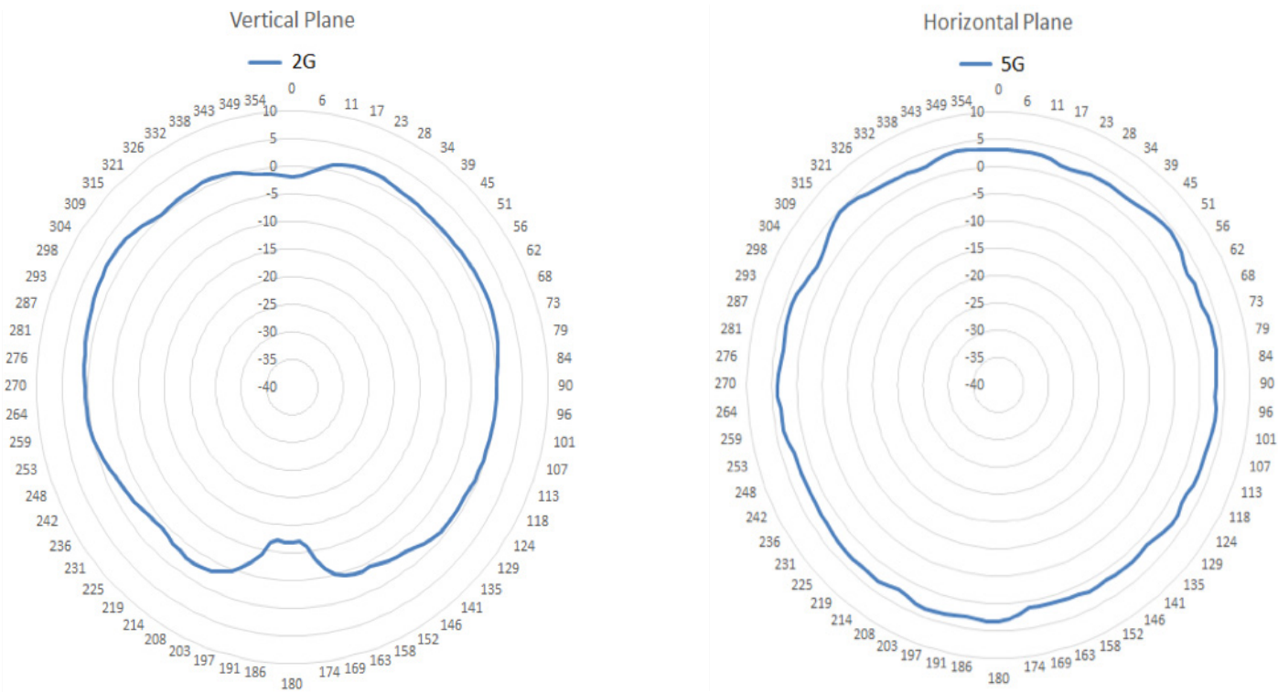
AP 505i Antenna Radiation Patterns — 2.4GHz
