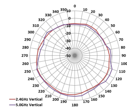
E-Plane Pattern
