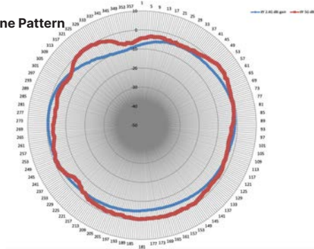
E-Plane Pattern
