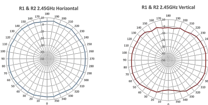
FAP-433G Radio 1&2 antenna plots
