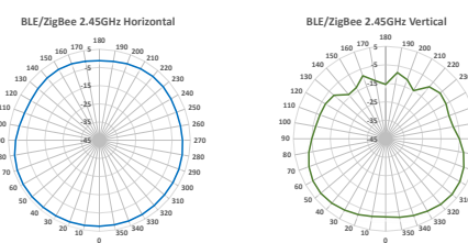
FAP-433G BLE/ZigBee antenna plots
